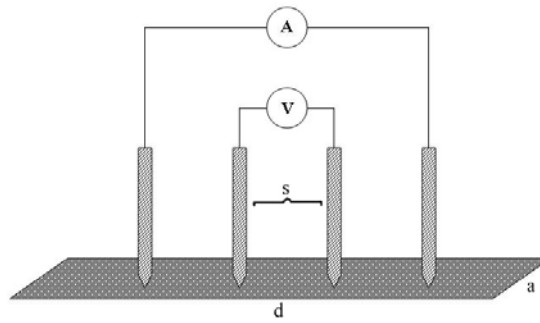
Fig. 6. Four probe geometry for thin film electric resistivity.
