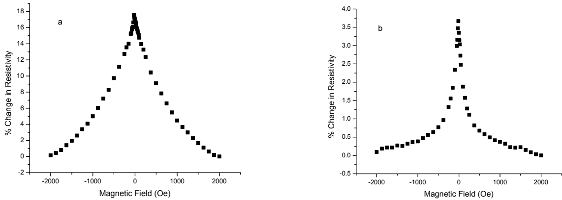
Fig. 7. Variation of electric resistivity as a function of applied magnetic field for: a) Co/Cu, and b) Ni/Cu multilayer.
